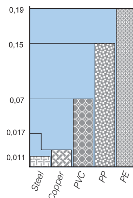
Graph A Linear thermal expansion expressed in mm. x m. x °C
